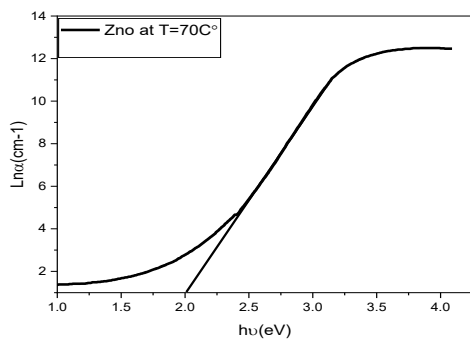
Figure 9. shows (\ln(\alpha)) versus (h\nu) at 70°C.
