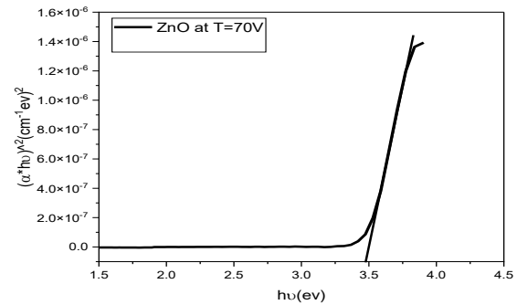
Figure 6. The optical energy gap curve of a ZnO sample deposited at a 70°C.
